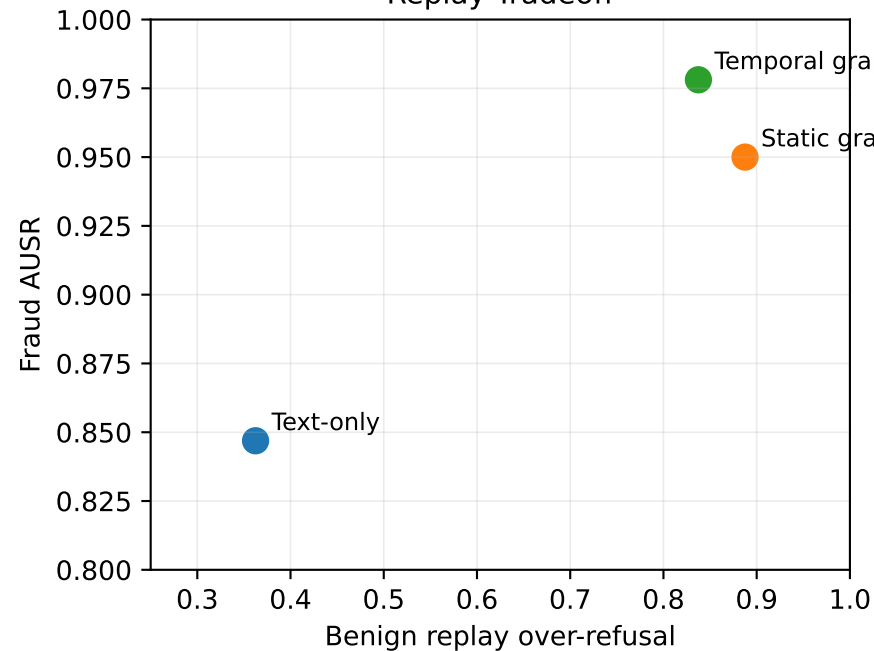
Replay Tradeoff
