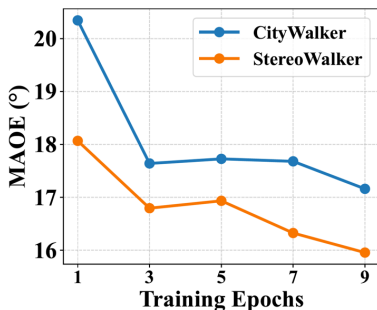
(c) Training efficiency (left) and navigation performance (right)
