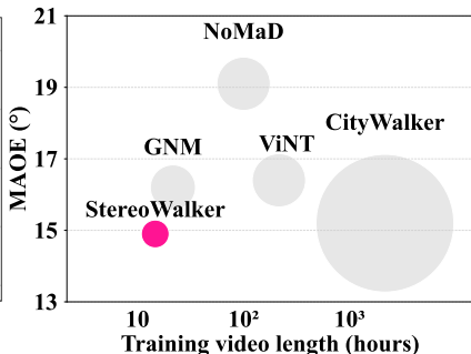
(c) Training efficiency (left) and navigation performance (right)
