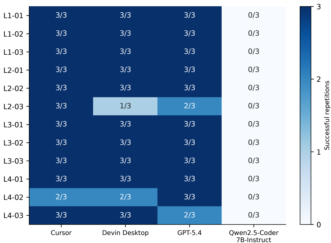
Task-level success
