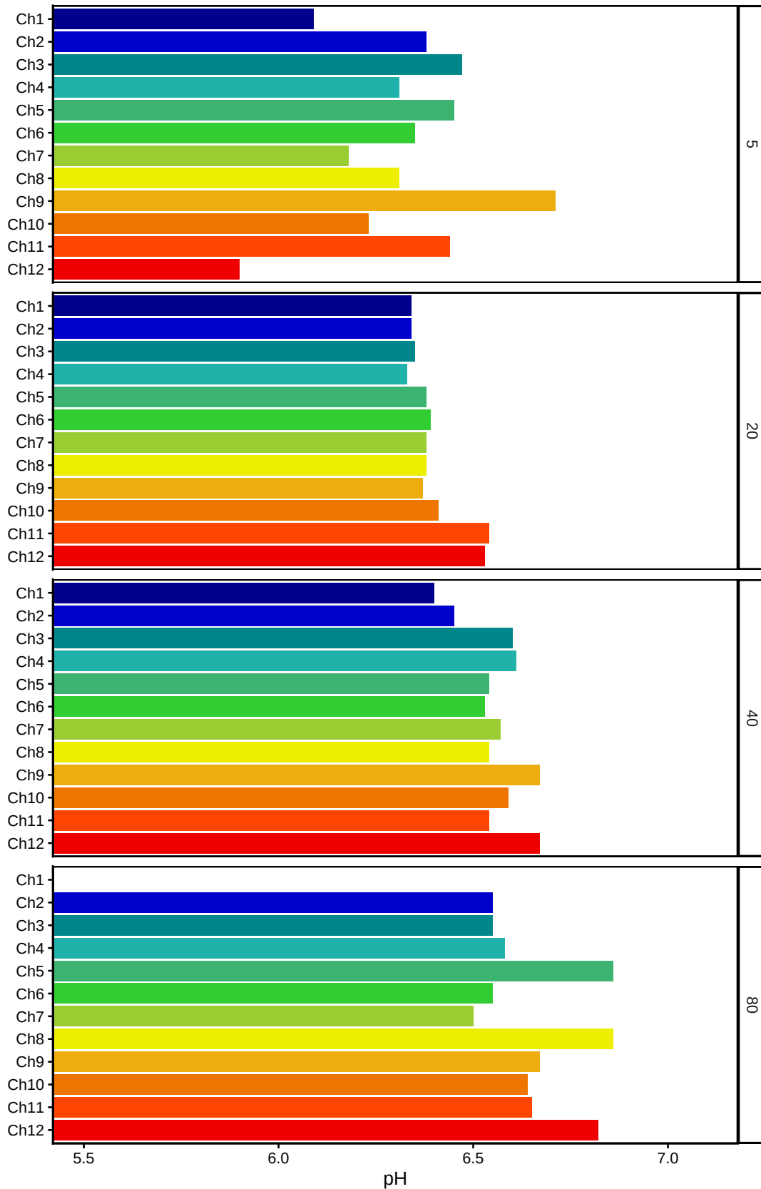
GENX: Porewater pH
