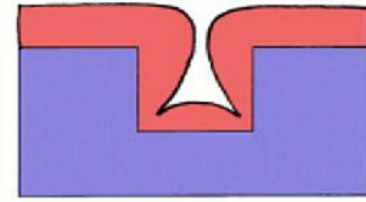
LPCVD, sputtering
