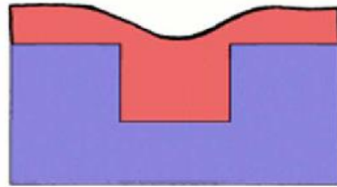
High-E sputtering (redeposition, high surface mobility)
