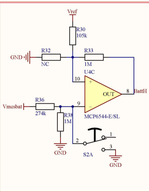
Control for battery high
