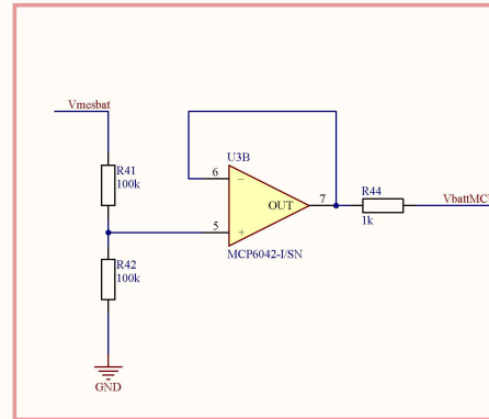
Divid by 2 the Vmesbatt
