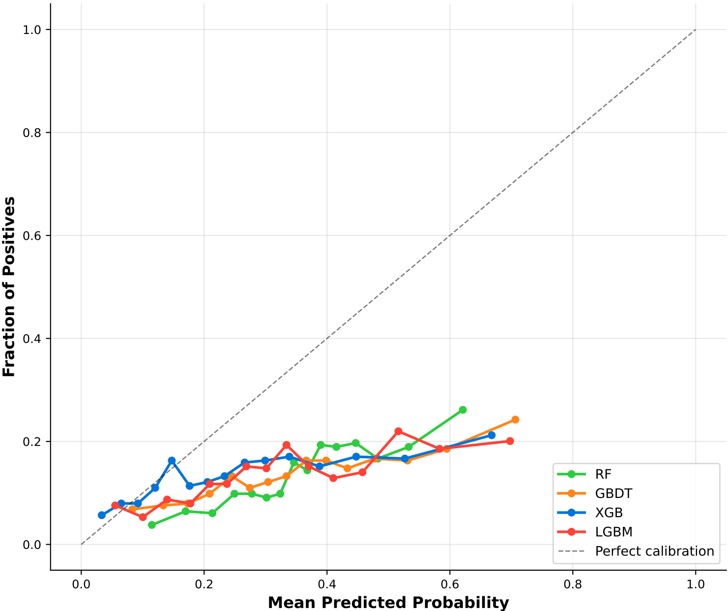
Calibration Curves (Reliability Diagrams)
