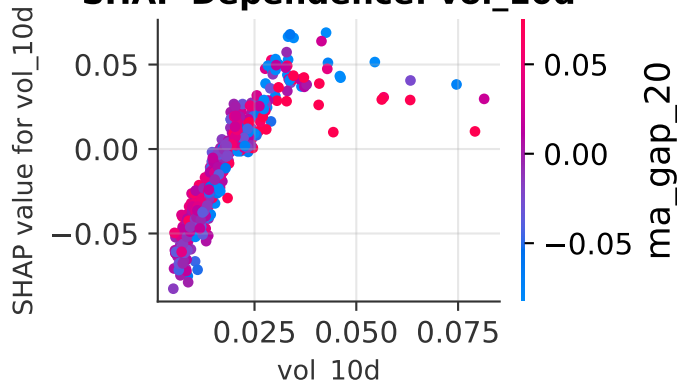
SHAP Dependence: vol_10d
