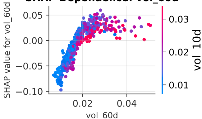
SHAP Dependence: vol_60d
