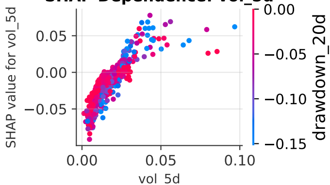
SHAP Dependence: vol_5d
