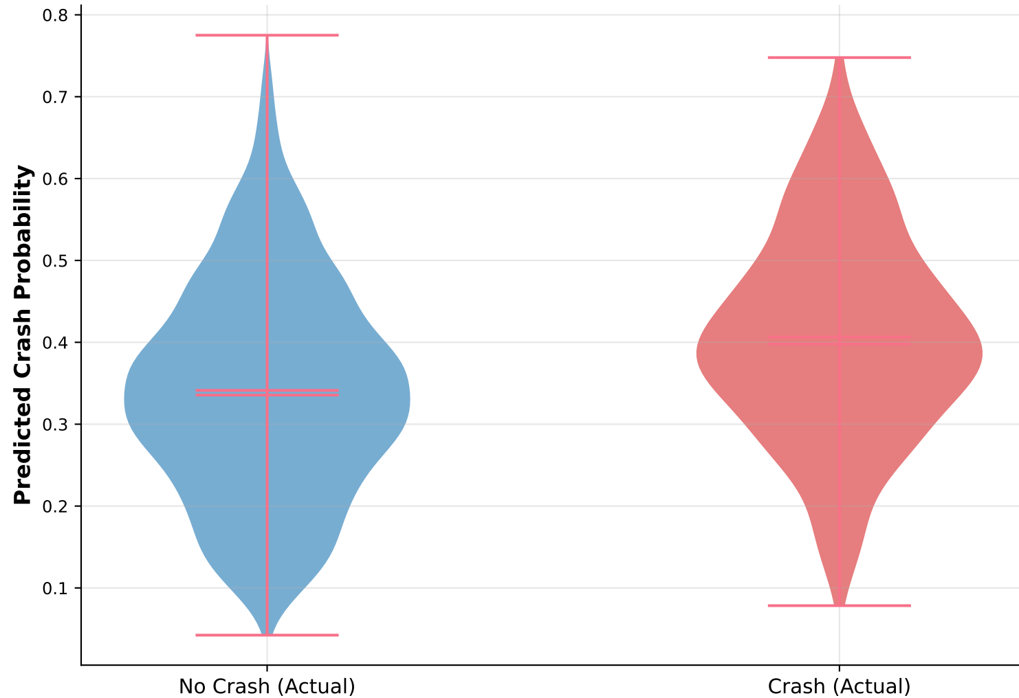
Prediction Distribution by True Class (RF)
