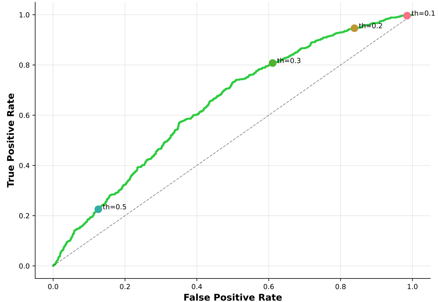
ROC with Threshold Annotations (RF, AUC=0.6413)
