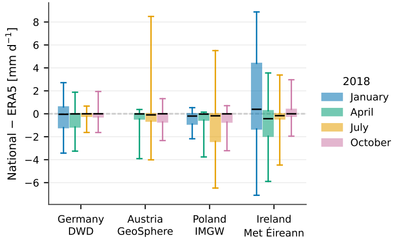
(b) Precipitation
