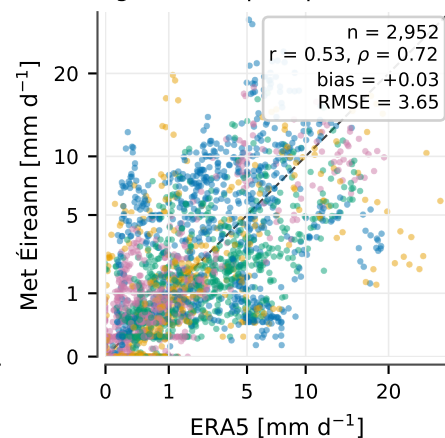
(g) Ireland: precipitation
