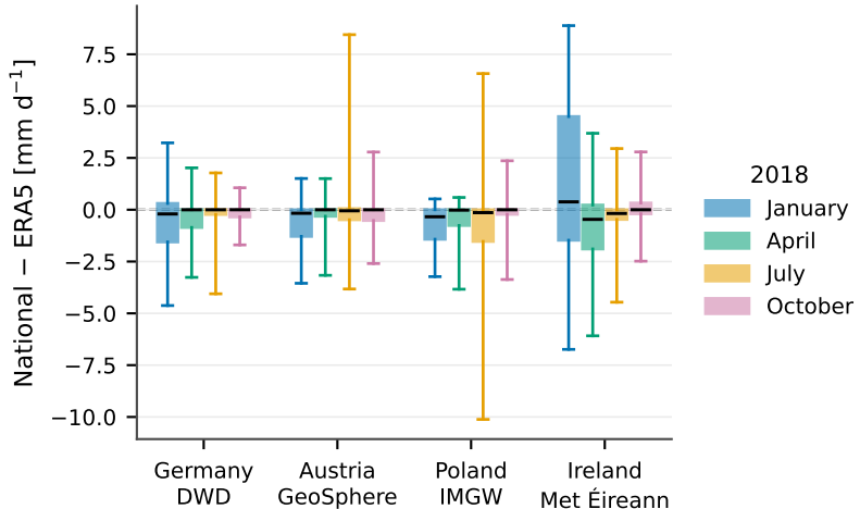
(b) Precipitation
