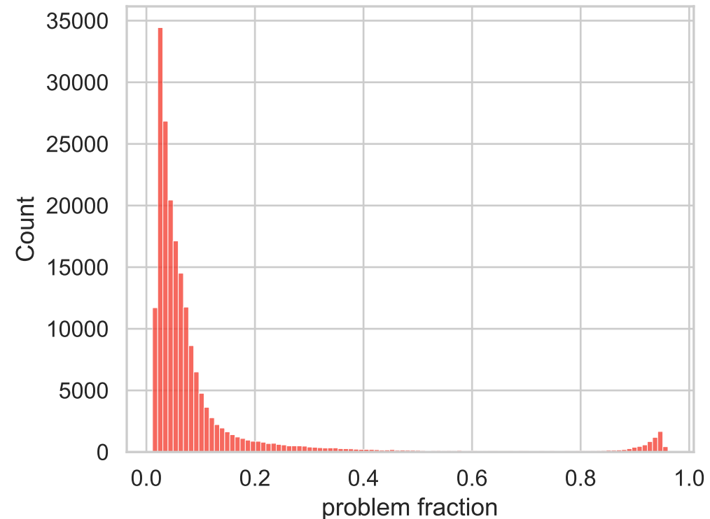
problem median=0.052
