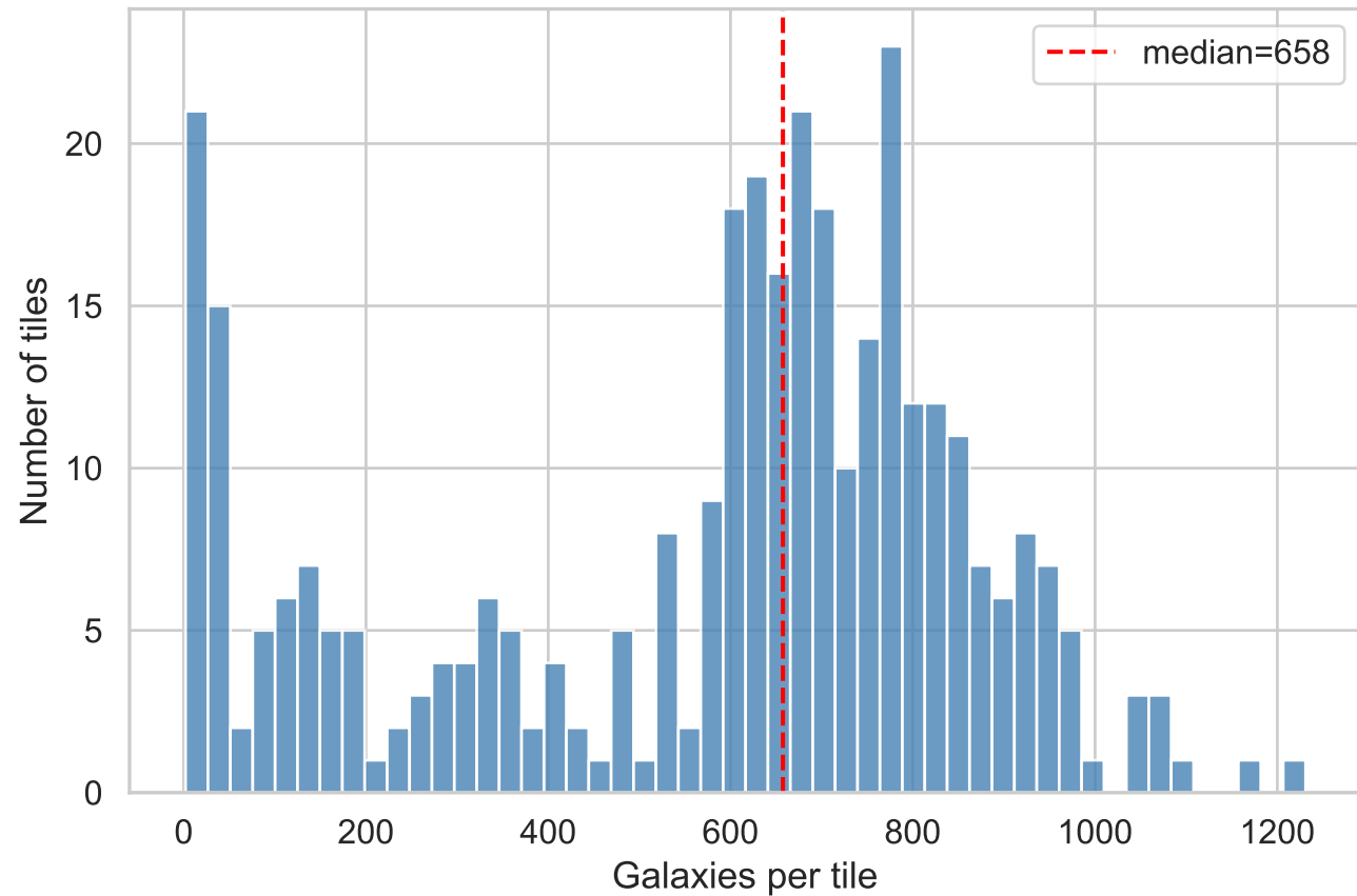
Galaxy Count per Tile (342 tiles)
