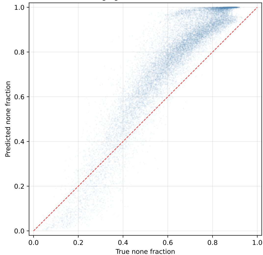
has-spiral-arms (r=0.934, N=6,188)
