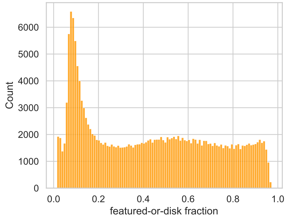
featured-or-disk median=0.410
