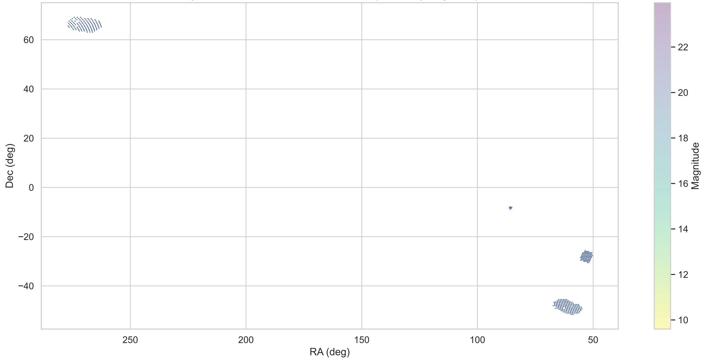
Sky Distribution of 195,716 Good Galaxies (colored by magnitude)
