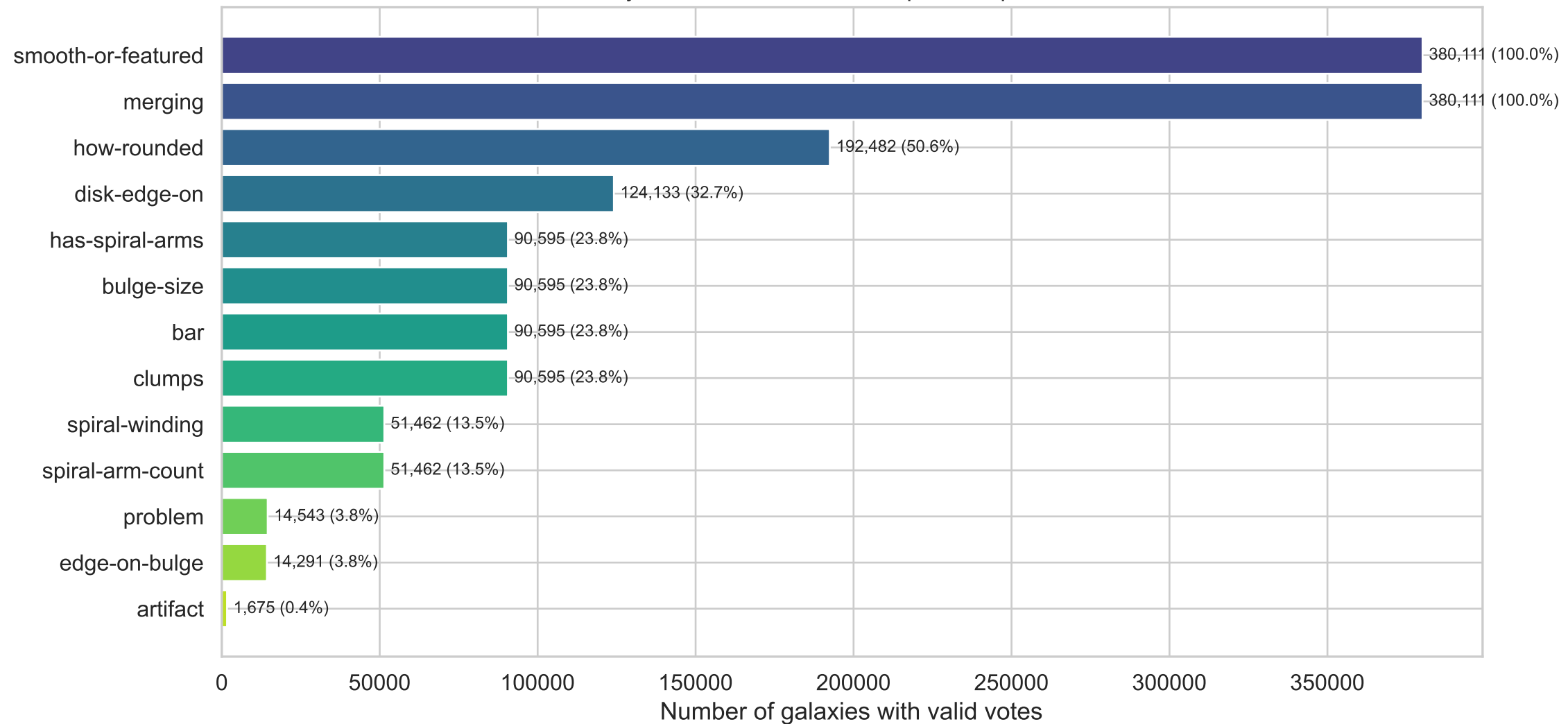
Galaxy Zoo Decision Tree: Sample Size per Question
