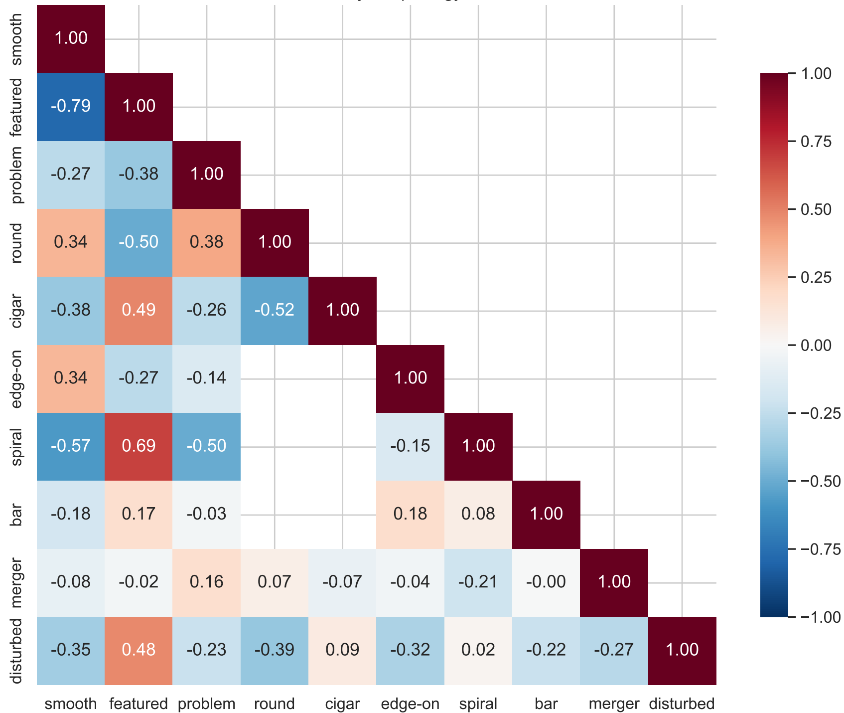
Correlation Between Key Morphology Vote Fractions
