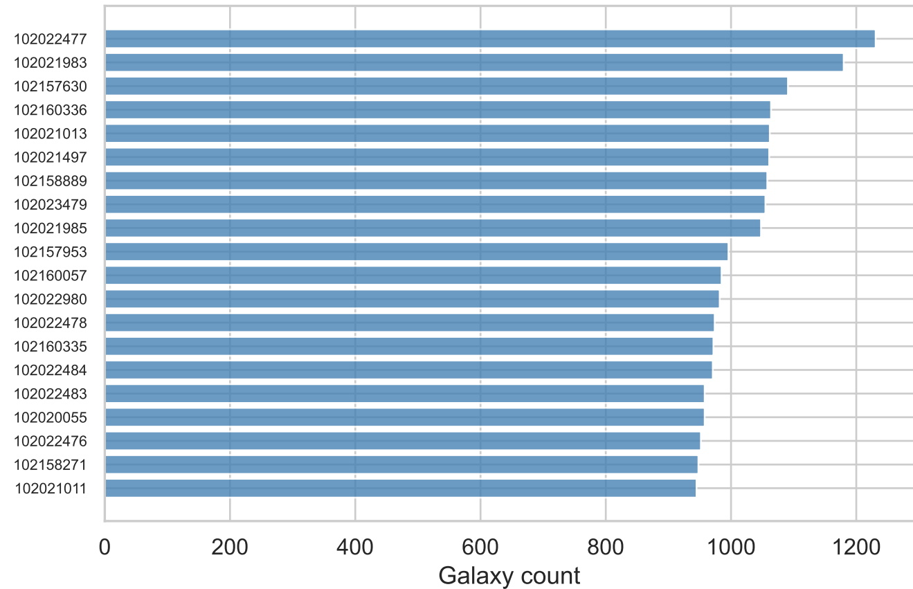
Top 20 Tiles by Galaxy Count
