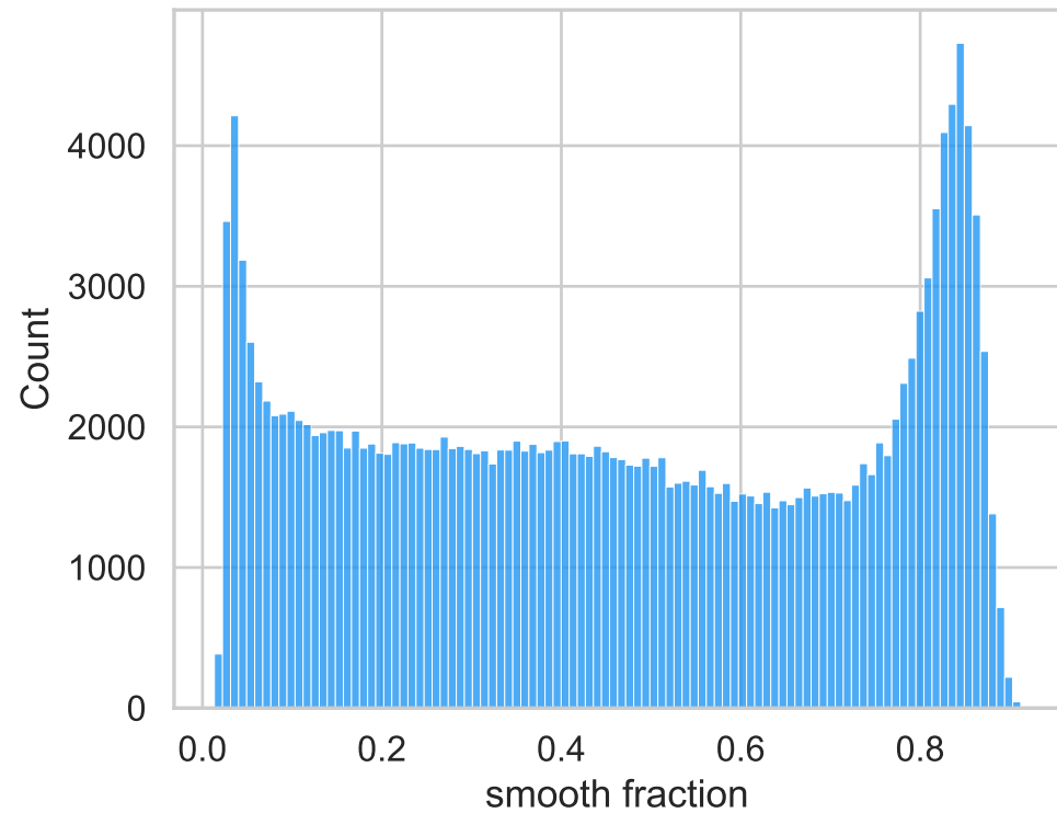
smooth median=0.455
