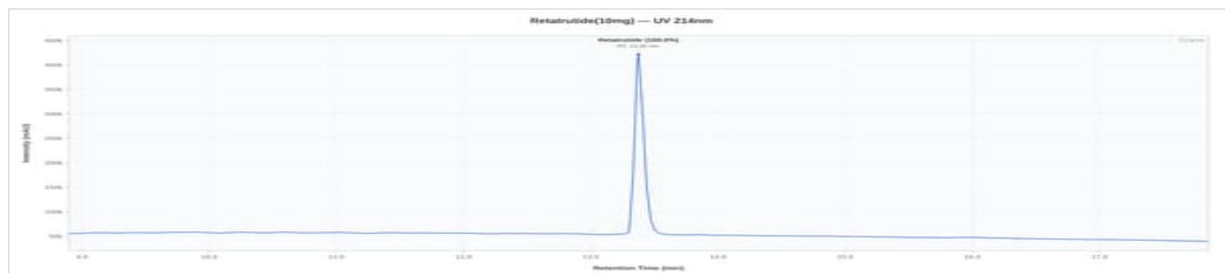
Retatrutide 10mg - RTA10-001: UV Chromatogram
