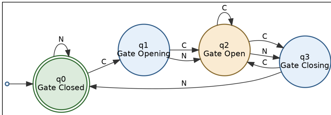
Fig. 1 — NFA state diagram for the Smart Parking Gate System (double circle = accepting state; the two outgoing C-edges from q_2 show the required non-determinism).
