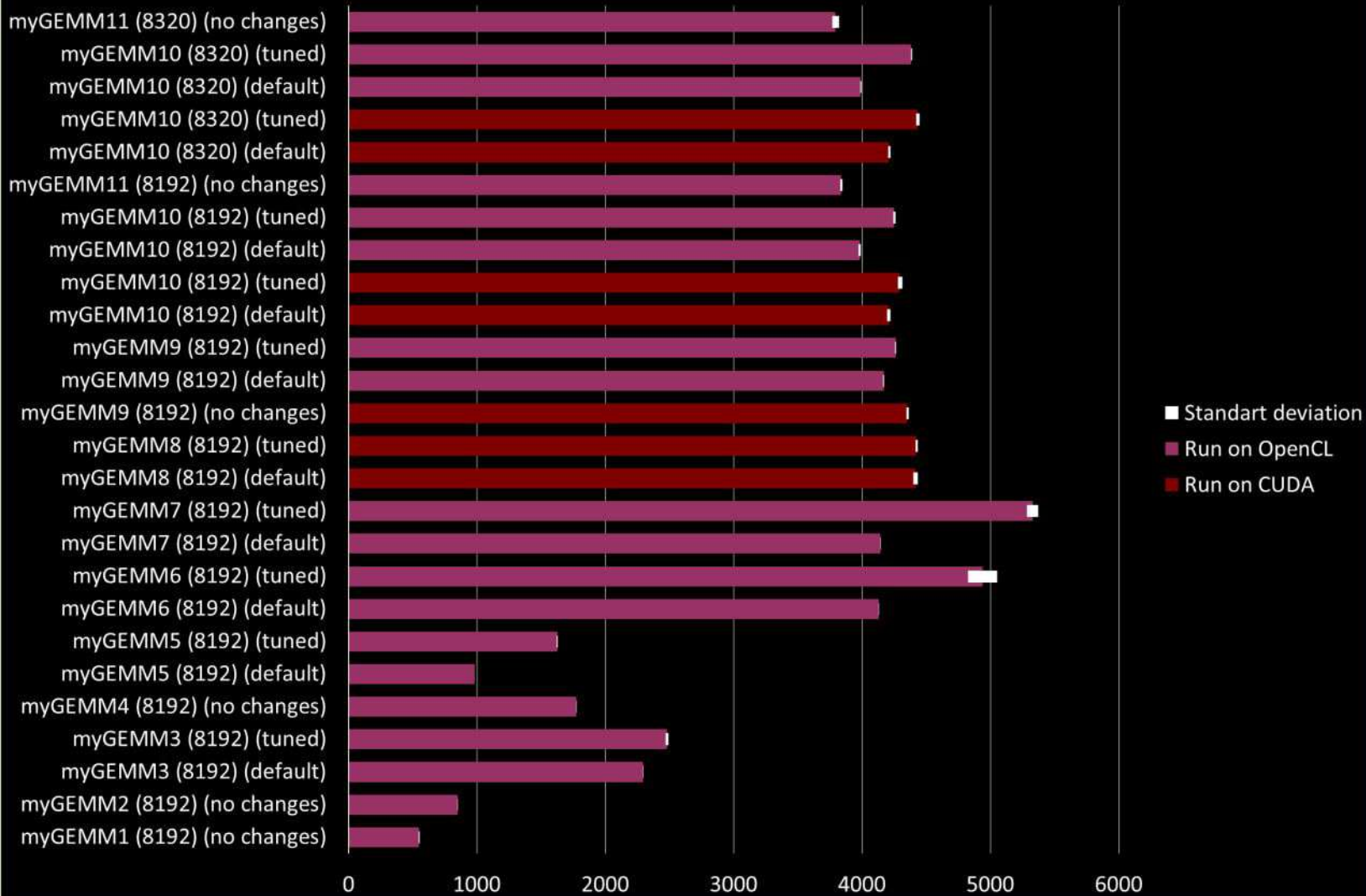
GFLOPS (8192x8192x8192 and 8320x8320x8320 on NVIDIA GeForce RTX 4060 Laptop GPU)
