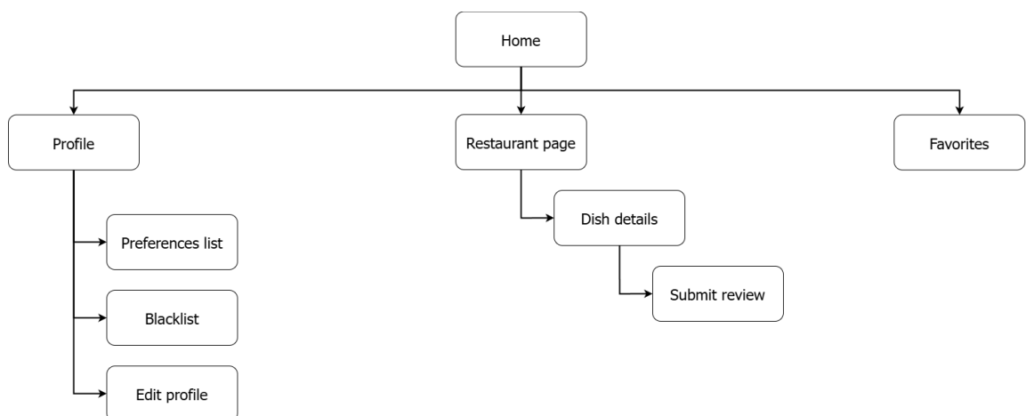
Figure 3.4: Site Map
