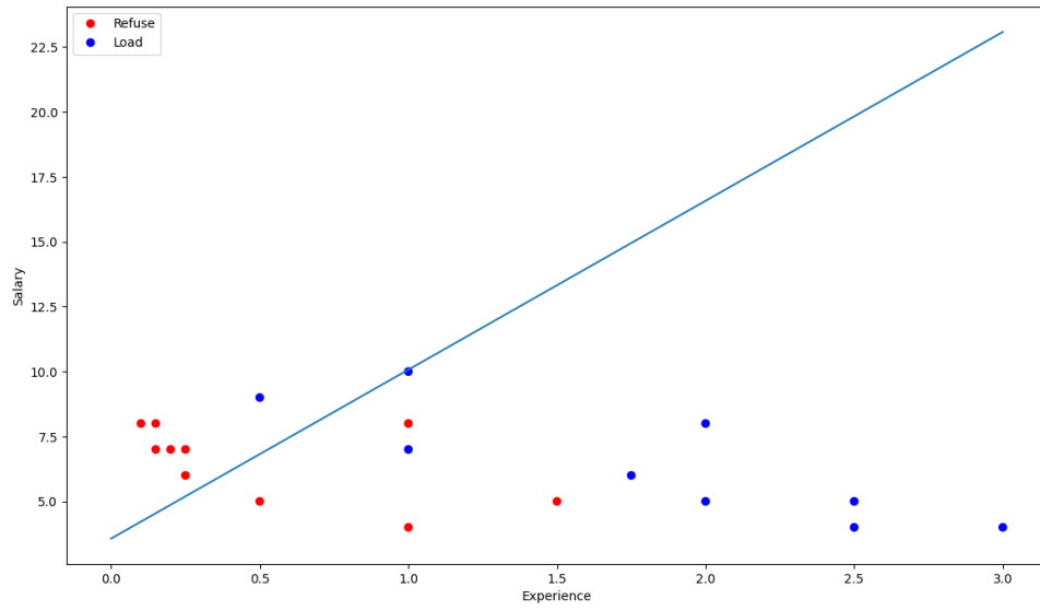
Figure 1: Predicted line
