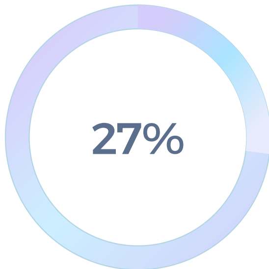
Subscribed Customers
