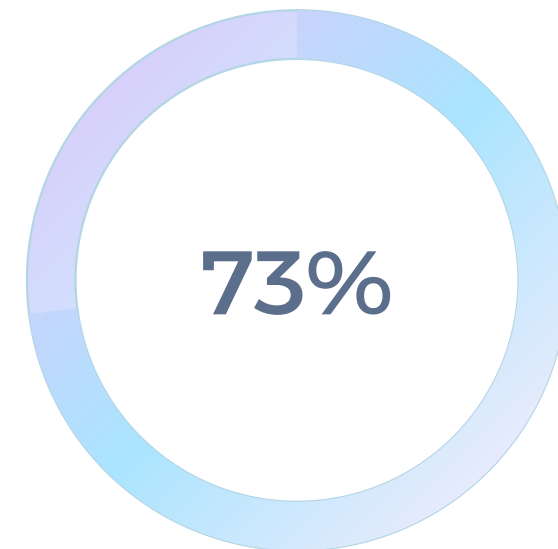
Non-Subscribed Customers
