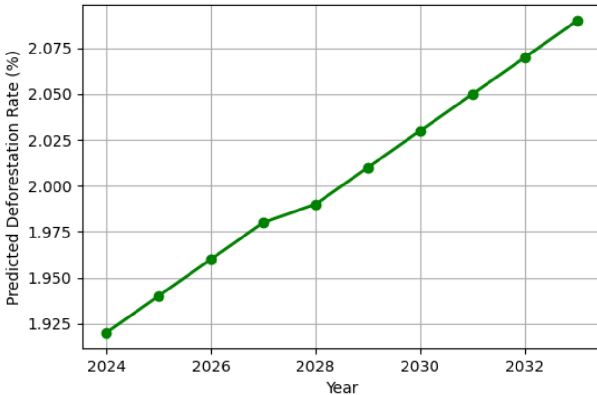
Predicted Deforestation (Next 10 Years) - Cooch Behar
