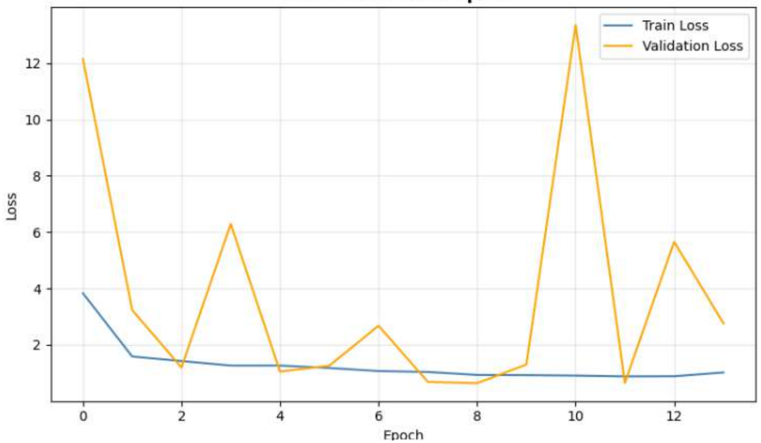
CNN — Loss over Epochs
