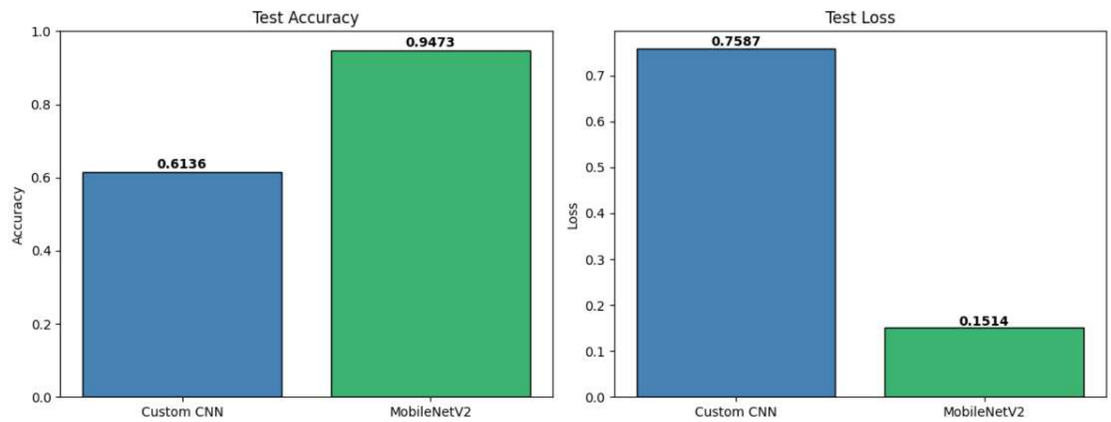
CNN vs MobileNetV2 — Performance Comparison
