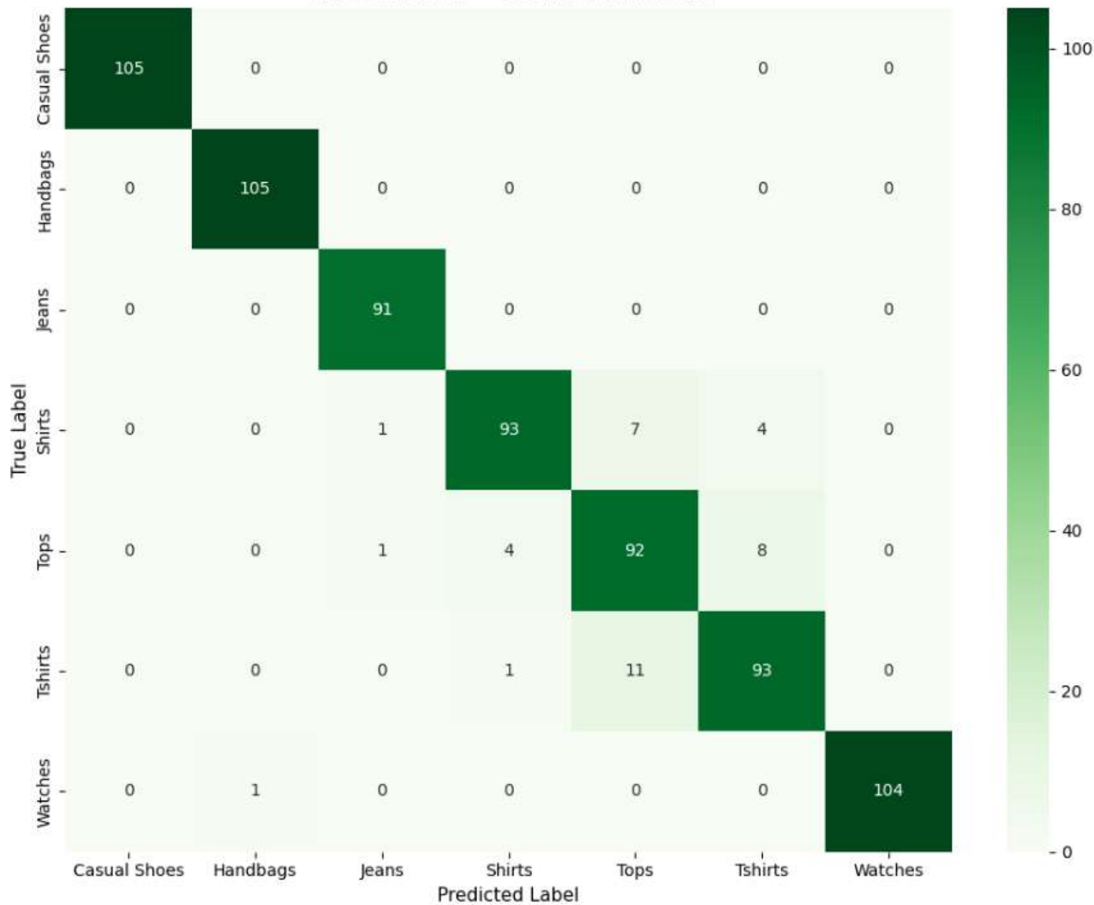
MobileNetV2 — Confusion Matrix
