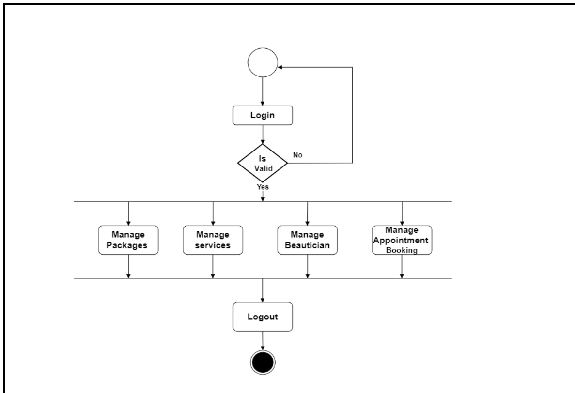
Figure 3.8 Activity Diagram of Admin
