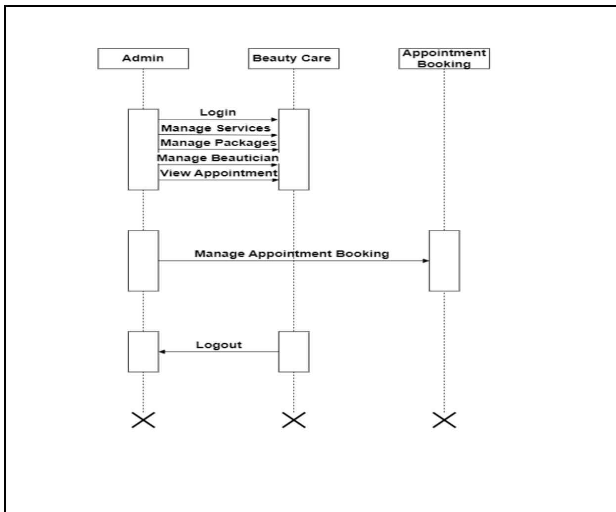
Figure 3.5 Interaction Diagram of Admin
