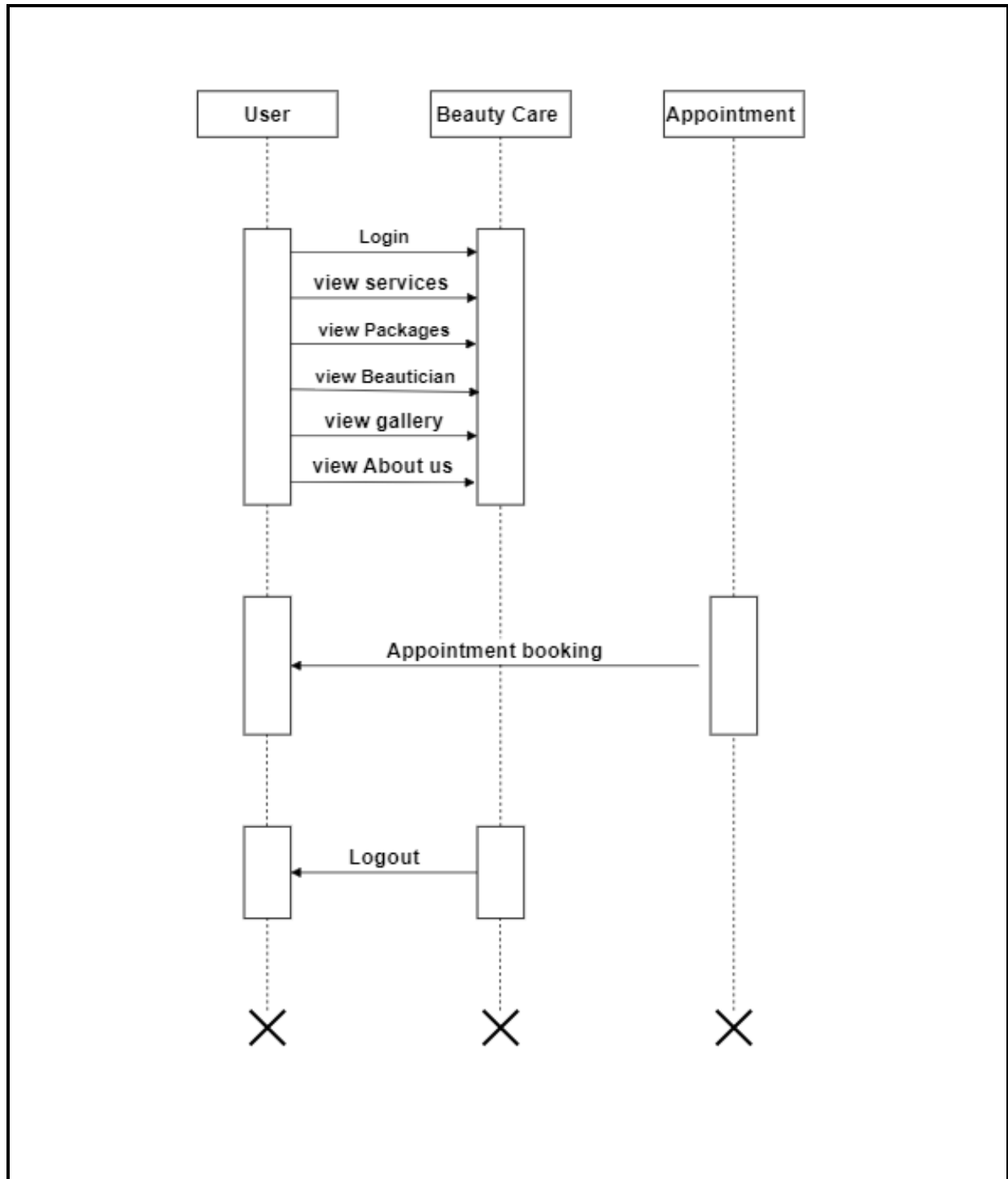
Figure 3.6 Interaction Diagram of Use
