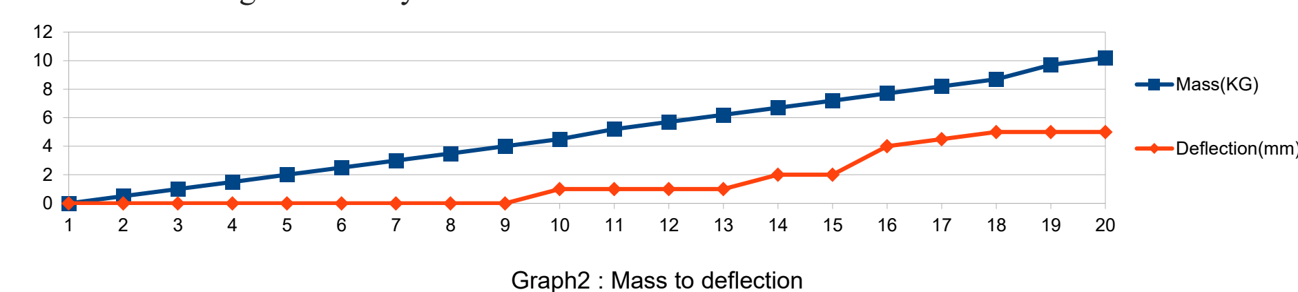
Graph2: Mass to deflection
