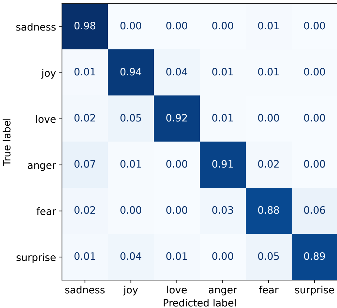
Normalized confusion matrix
