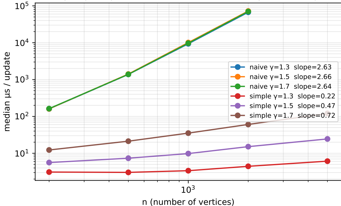
Fig 5: per-update time vs n on Erdős-Rényi ( m \approx n^\gamma )
