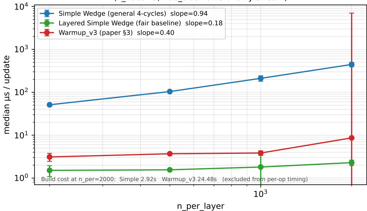
Fig 8: per-update time on planted-hub layered graphs ( k\_hubs=5 , hub\_bias=0.75 D-only stream)
