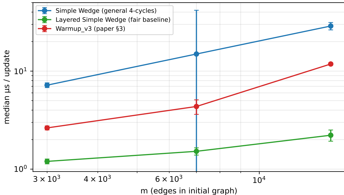
Fig 8b: robustness on no-hub layered graphs ( k_{\text{hubs}}=0 , uniform-random D-stream — no class structure to exploit)
