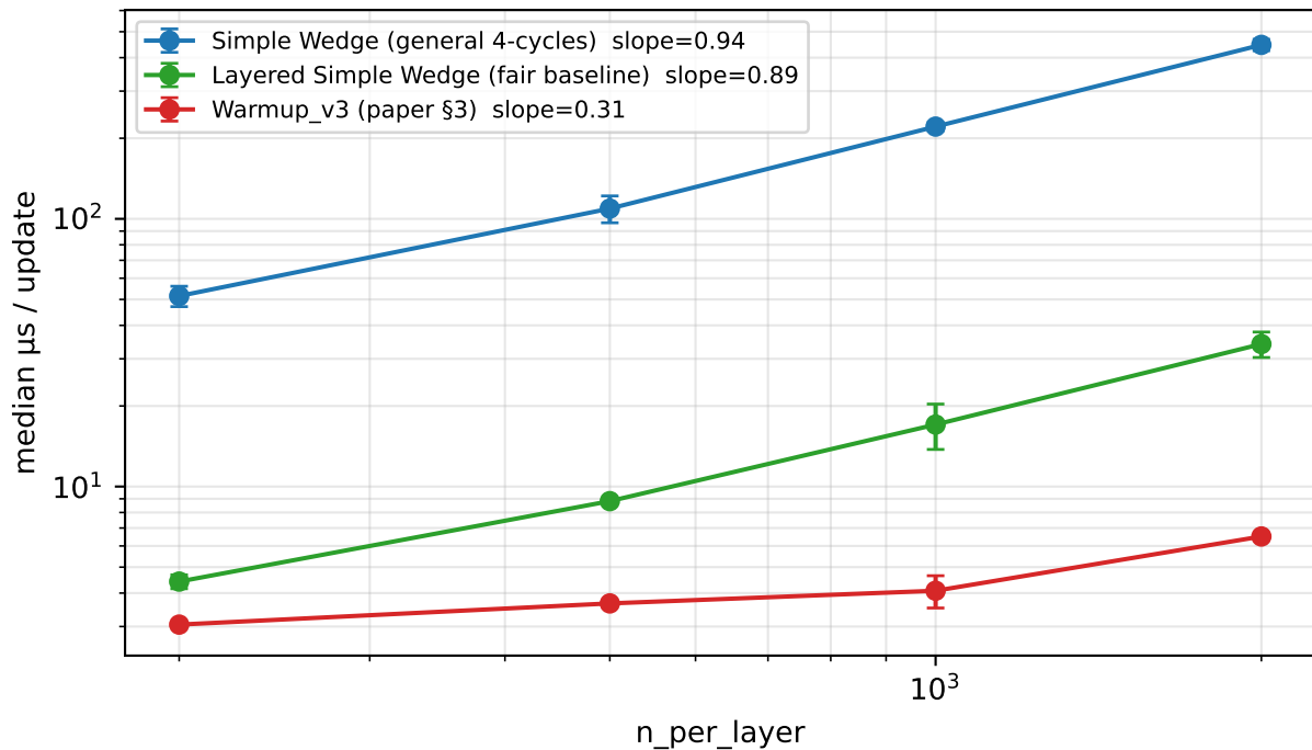
Fig 8c: bilateral-hub graphs — HH-query regime ( k_{\text{hubs}}=5 in BOTH L1 and L4, \text{hub\_bias}=0.85 )
