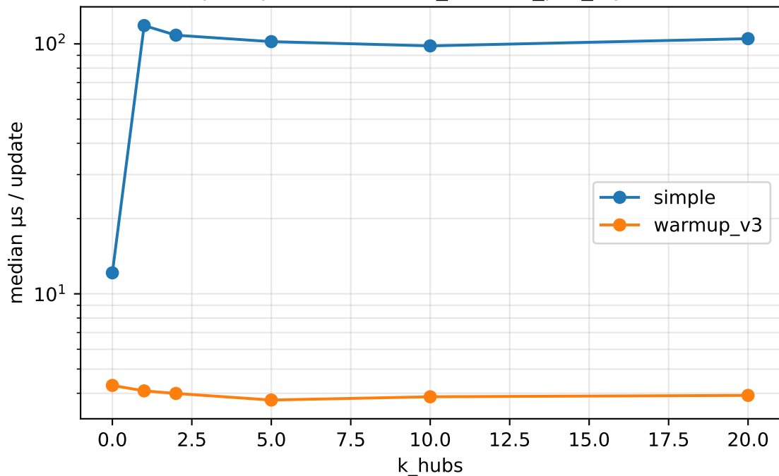
§3.7: per-update time vs k_hubs (n_per_layer=500)
