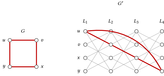
Figure 2: Lifting a general graph G (left) to a 4-layered graph G' (right). Every vertex of V is replicated in each layer L_1, \dots, L_4 ; gray edges schematically depict the lifted copies between consecutive layers. The 4-cycle u, v, x, y in G corresponds to the highlighted layered 4-cycle (u, 1) \rightarrow (v, 2) \rightarrow (x, 3) \rightarrow (y, 4) \rightarrow (u, 1) , with the closing L_4 \rightarrow L_1 edge drawn as a curved arc. For legibility, only the highlighted cycle is shown in full; remaining lifted edges are partial.
