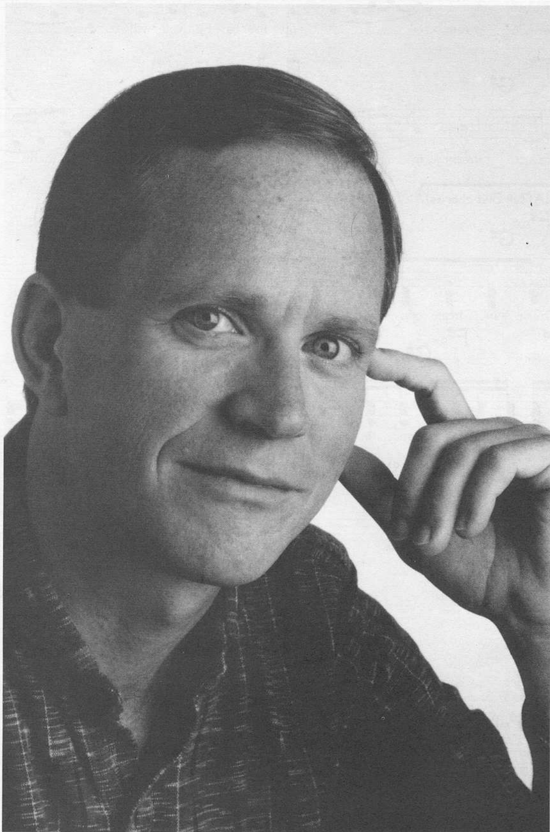
SKY EVERGREEN
