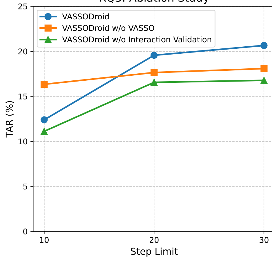
RQ3: Ablation Study
