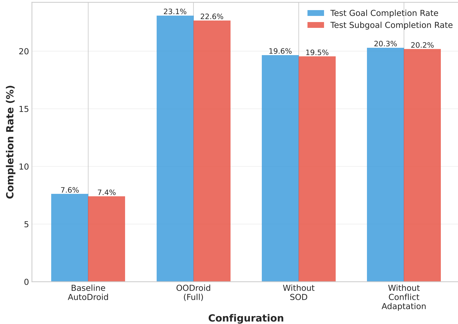
Test Goal and Subgoal Completion Rates
