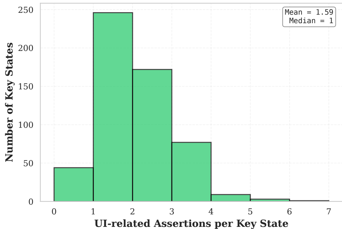
UI-related Assertions Distribution
