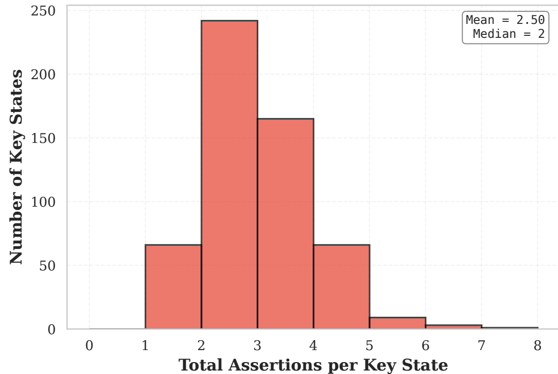
Total Assertions Distribution
