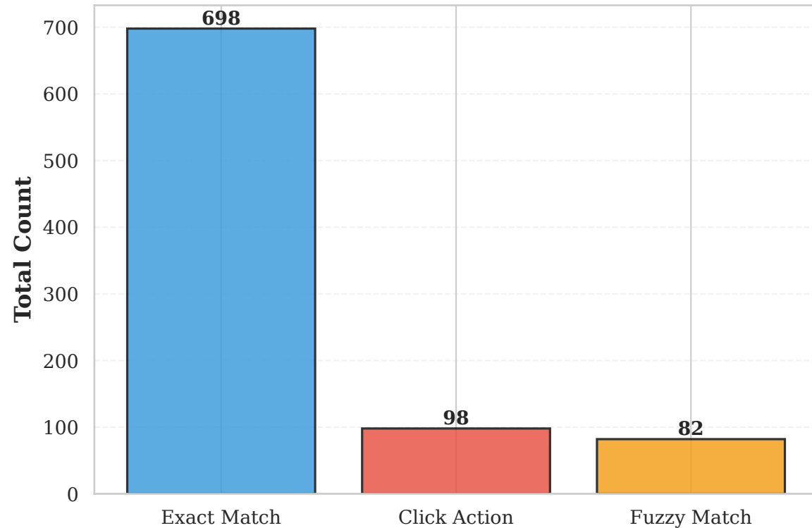
UI Assertion Types
