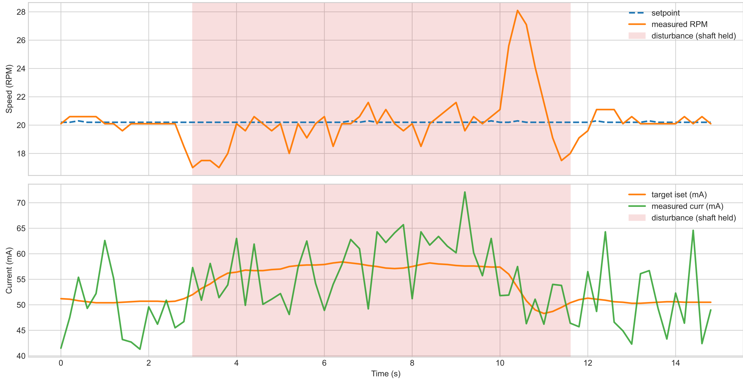
Manual disturbance test — speed and current response (setpoint 20.2 RPM)
