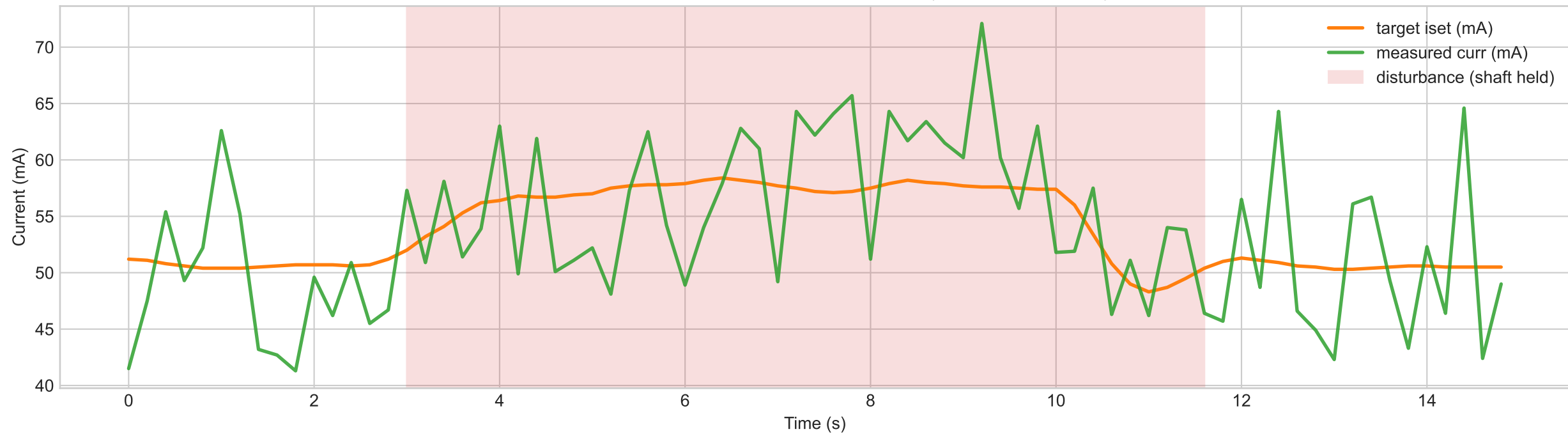
Manual disturbance test — current response (setpoint 20.2 RPM)
