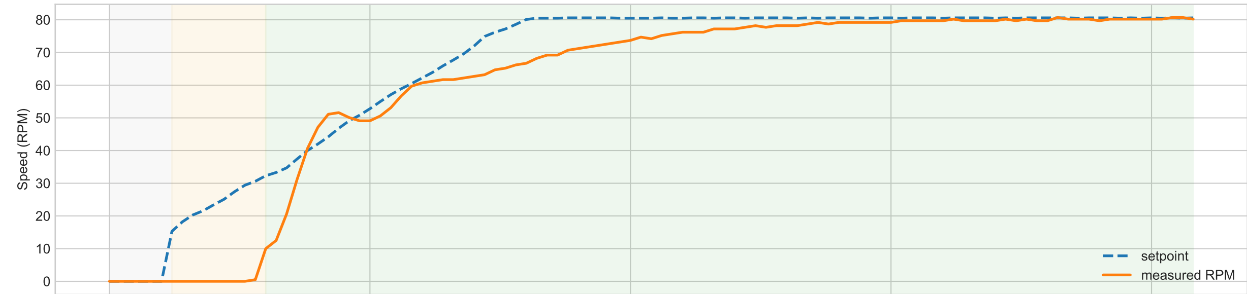
Slow ramp to 80 RPM — speed tracking
