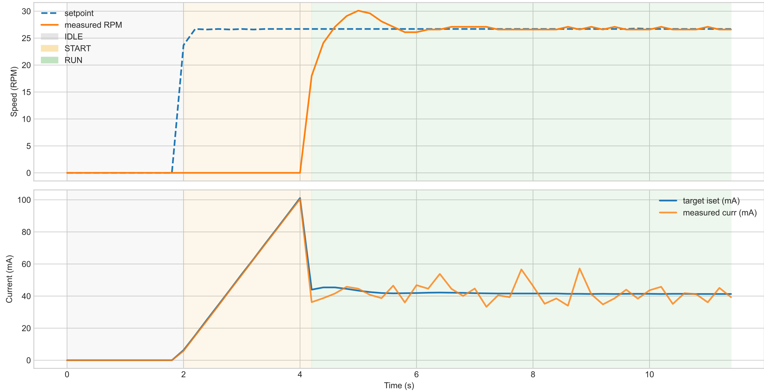
Low-speed startup — speed and current
