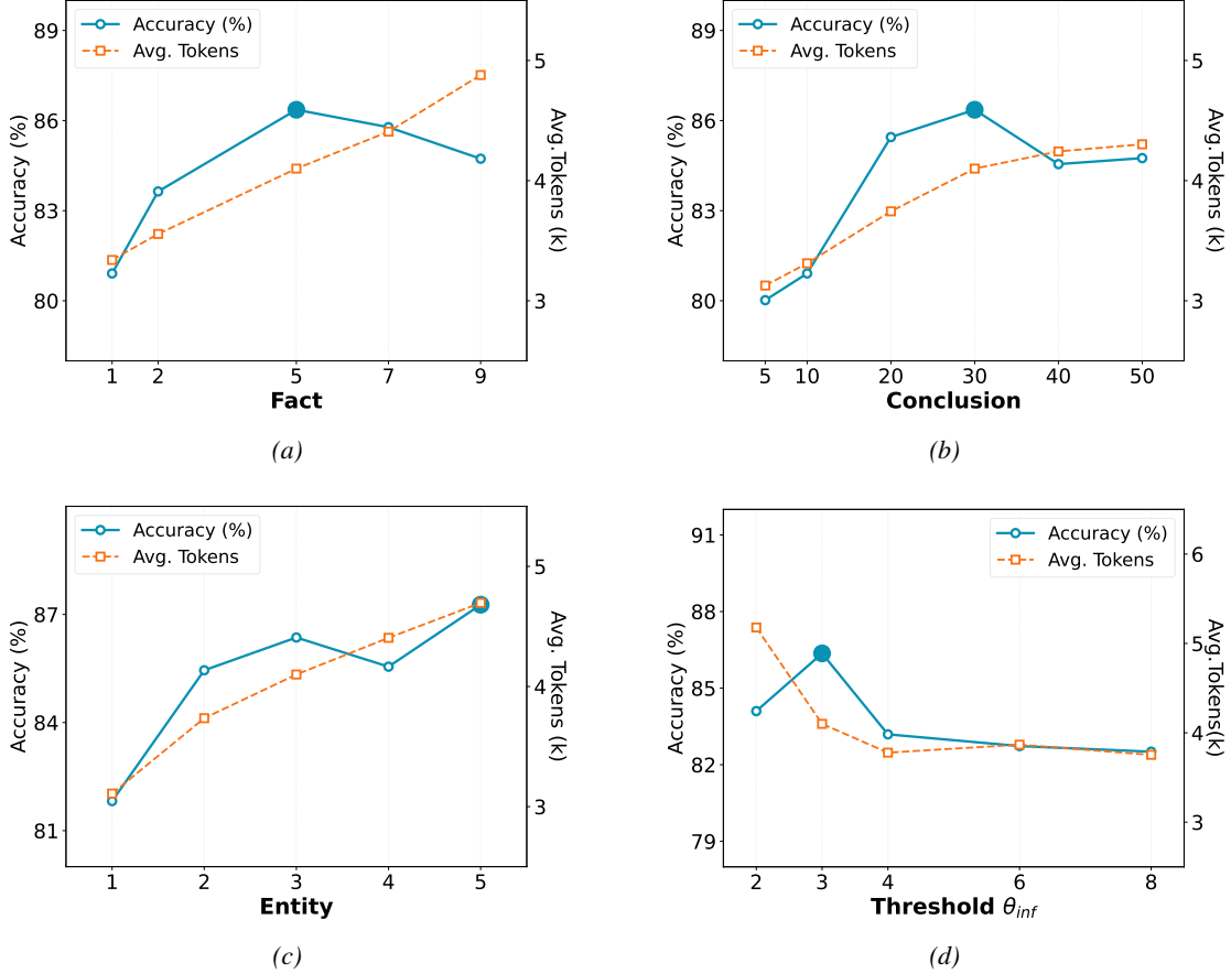
Figure 8. Parameter sensitivity analysis for RGMem’s retrieval and dynamics parameters.
