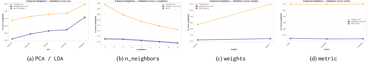
Fig. 8. Iterative validation curves for KNN highlighting the impact of supervised LDA projection and distance metrics.
