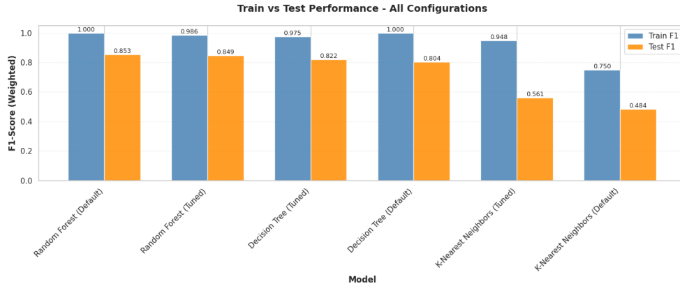
Fig. 10. Visual comparison of Weighted F1-Score on training and test sets across all six evaluated models.
