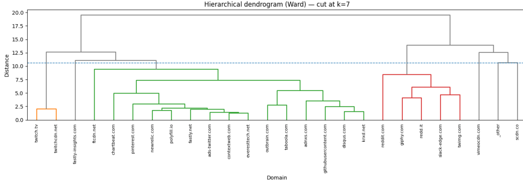
Fig. 14. Ward hierarchical clustering cut at approximately k = 7 .
