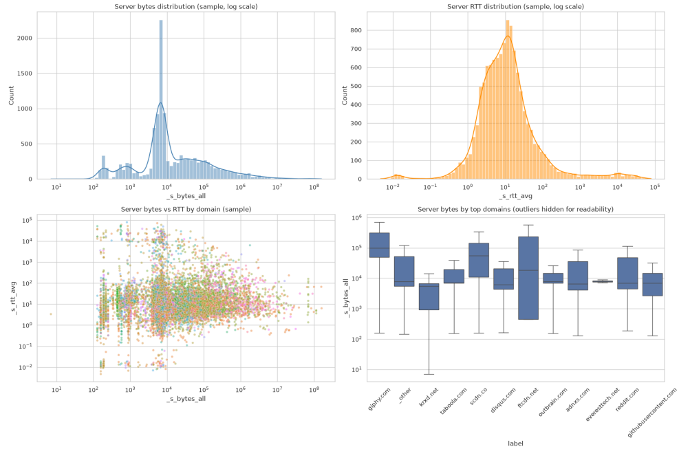
Fig. 2. Top: log-scale histograms of server bytes and server RTT (12k-flow sample). Bottom-left: server bytes vs. server RTT (log-log). Bottom-right: server bytes per flow for the 12 most frequent domains (outliers hidden).
