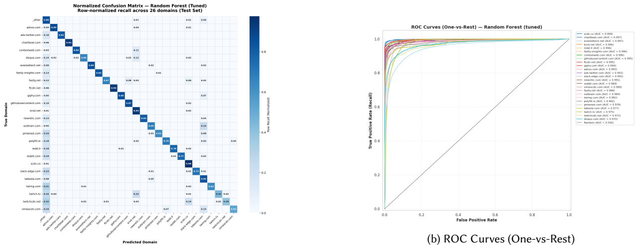
(a) Normalized Confusion Matrix (b) ROC Curves (One-vs-Rest) Fig. 9. Normalized confusion matrix and One-vs-Rest ROC curves across all 26 classes for the champion classifier.
