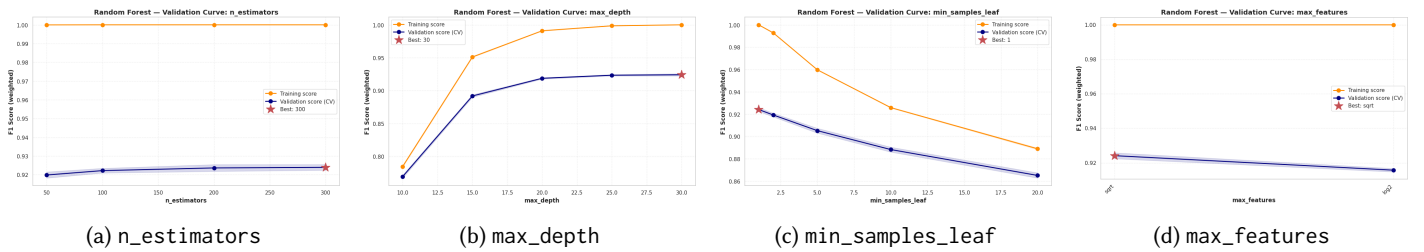
Fig. 6. Iterative validation curves for Random Forest across its four sequential hyper-parameters.
