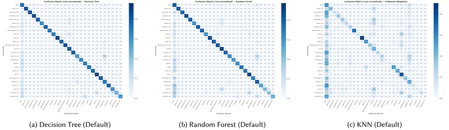
Fig. 5. Row-normalized test set confusion matrices for baseline classifiers under default hyper-parameters.
