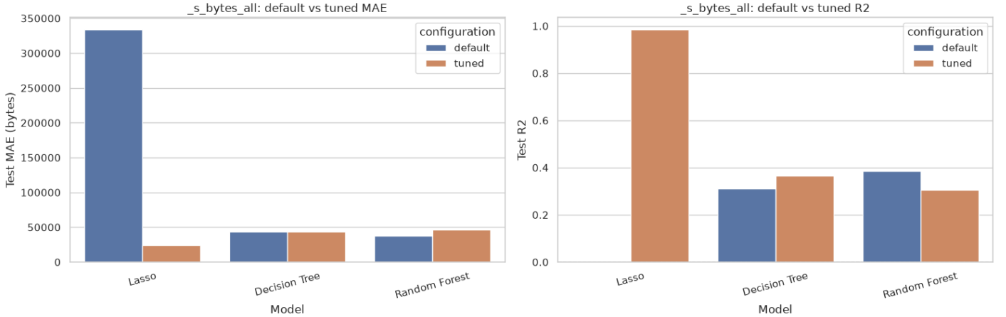
Figure 16: Default and tuned official-test performance for byte prediction. Weakening Lasso regularization produces the strongest test improvement, while both tuned tree-based models retain large train-test gaps.
