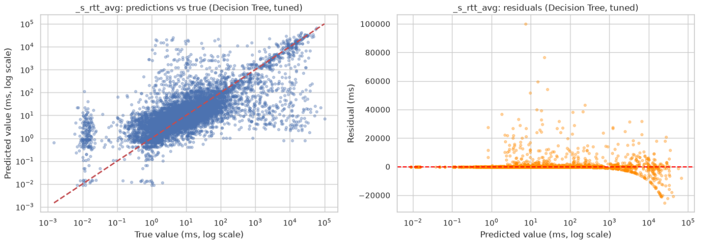
Figure 19: Official-test predictions and residuals for the CV-selected depth-16 RTT Decision Tree. Broad dispersion is consistent with limited latency information and the extreme upper tail.
