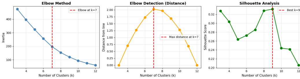
Fig. 11. K-Means model selection for random_state=15 : inertia, geometric elbow detection and Silhouette score.
