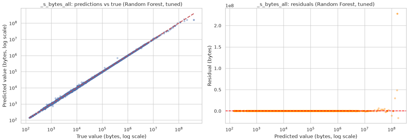
Figure 17: Official-test predictions and residuals for the CV-selected byte Random Forest. Rare upper-tail errors dominate RMSE and reduce R^2 .
