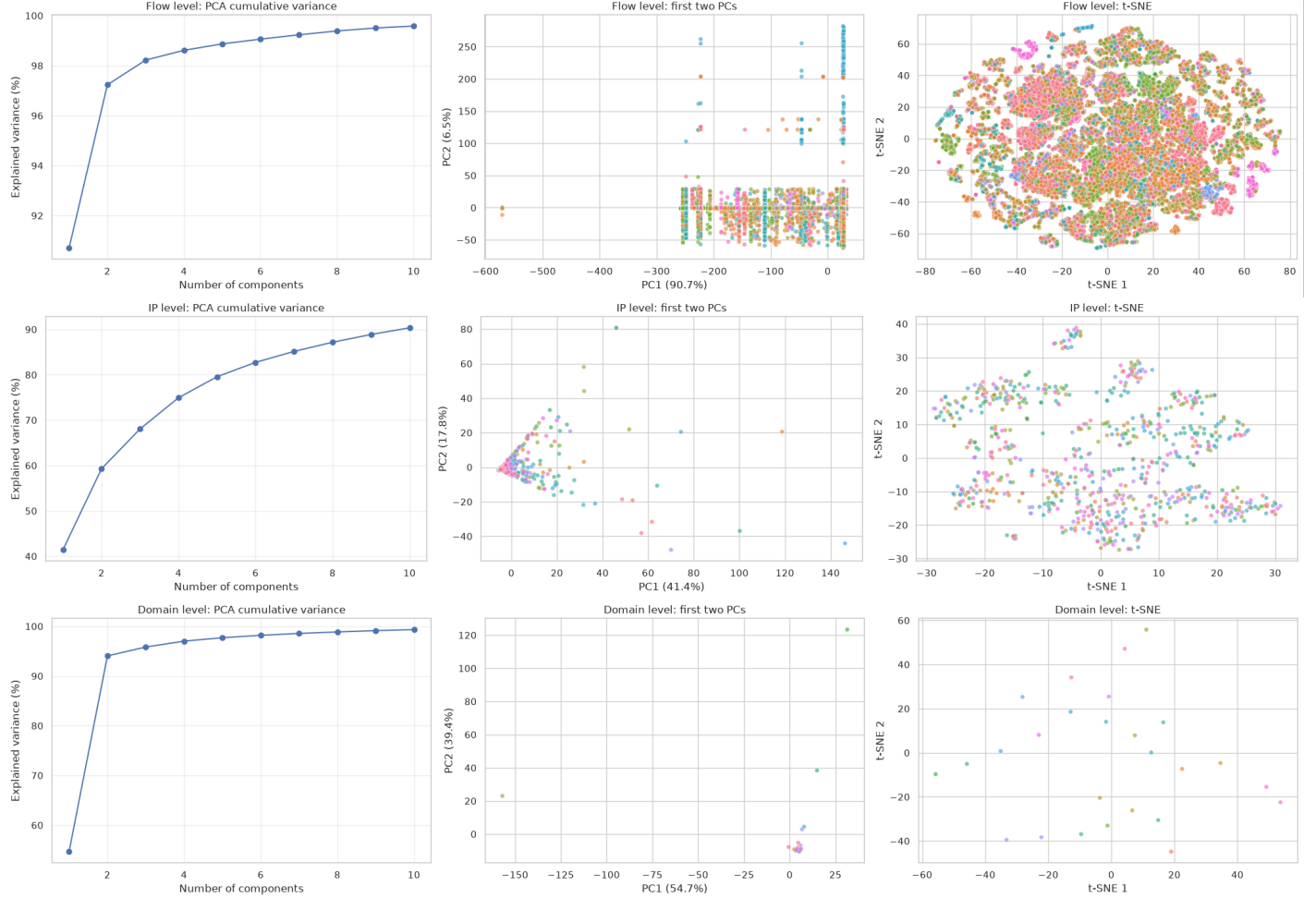
Fig. 4. PCA cumulative variance, first two PCs, t-SNE. (Top: flow level. Middle: IP level. Bottom: domain level)
