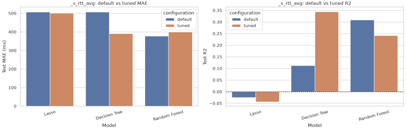
Figure 18: Default and tuned official-test RTT performance. Constraining the Decision Tree produces the clearest improvement, whereas Lasso remains underfit and tuned forest does not improve on default.
