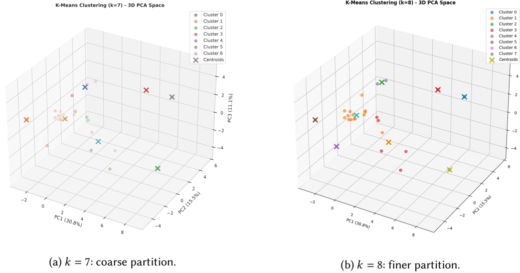
Fig. 13. Three-dimensional K-Means visualization in the PC1–PC2–PC3 space. Centroids are marked with crosses.
