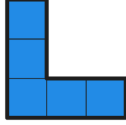
FIGURE 39. 5V pentomino
