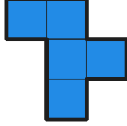
FIGURE 25. 5F pentomino
