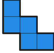
FIGURE 46. 5W pentomino
