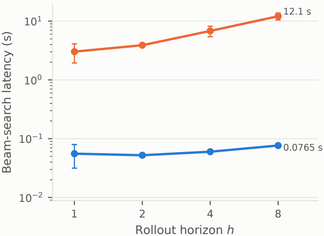
(a) HF Transformers
