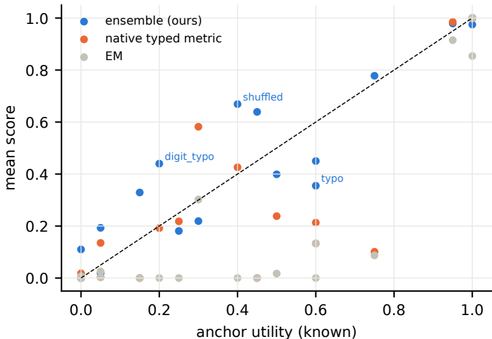
Score vs known utility per anchor operator
