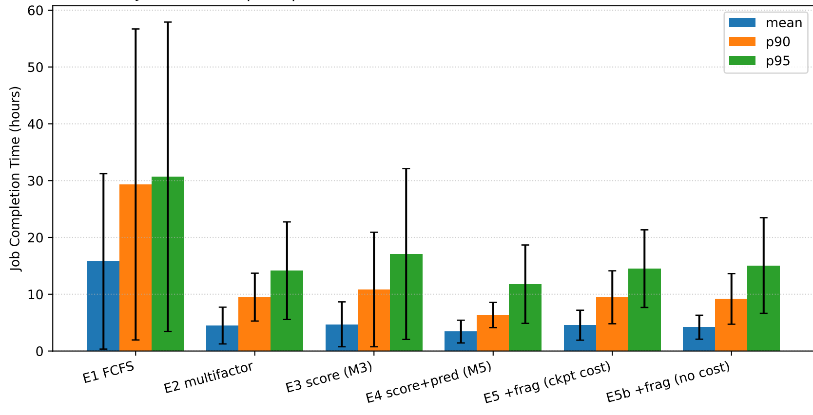
JCT — mean / p90 / p95 across schedulers (error bars = 95% CI, n=5 seeds)
