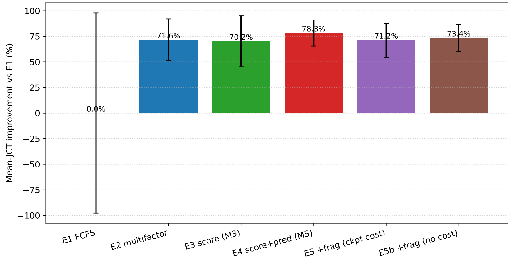
Mean-JCT reduction relative to FCFS baseline (95% CI, n=5 seeds)
