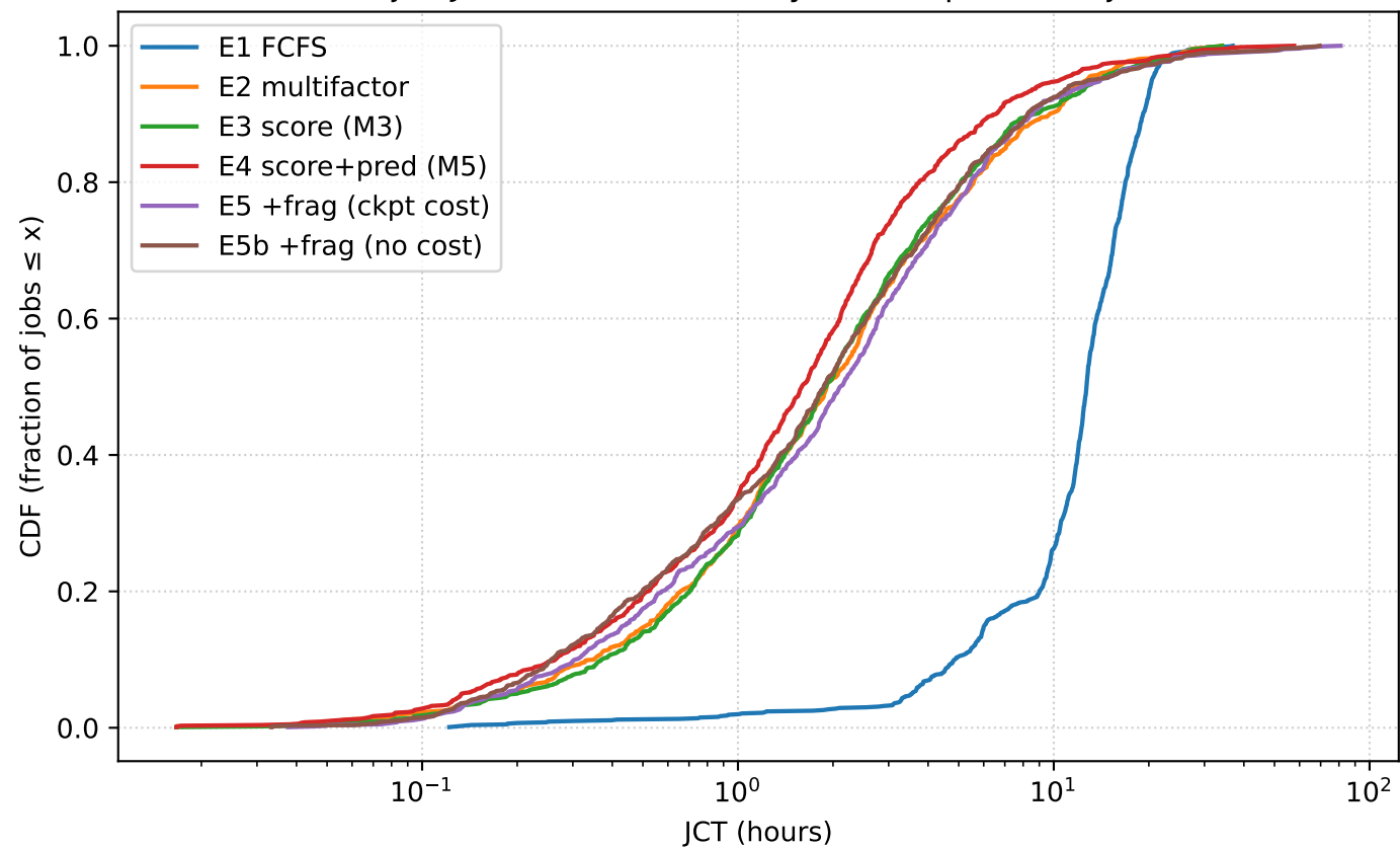
Per-job JCT distribution (Philly subsample, 1000 jobs)
