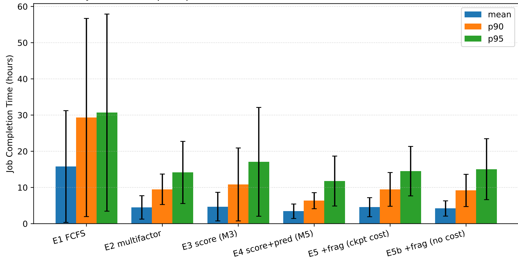
JCT — mean / p90 / p95 across schedulers (error bars = 95% CI, n=5 seeds)
